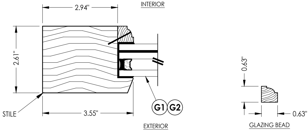
2 2 HORIZONTAL CROSS SECTION
