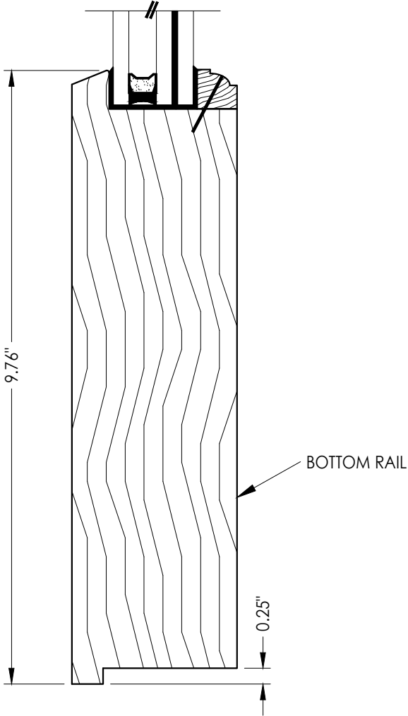
1 2 VERTICAL CROSS SECTION
