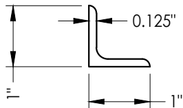
34 ALUM FLANGE
