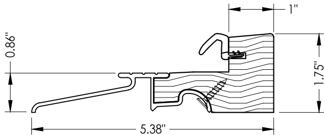
16 SILL (OUTSWING)
