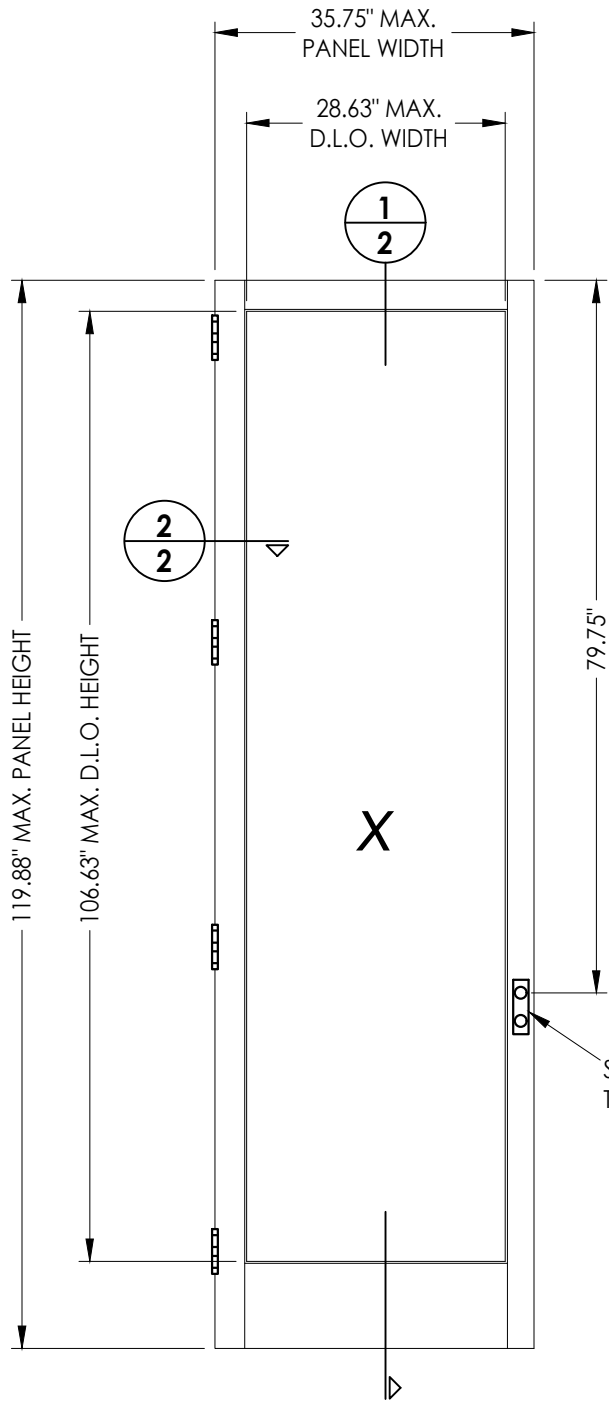
40 GLAZED DOOR PANEL
